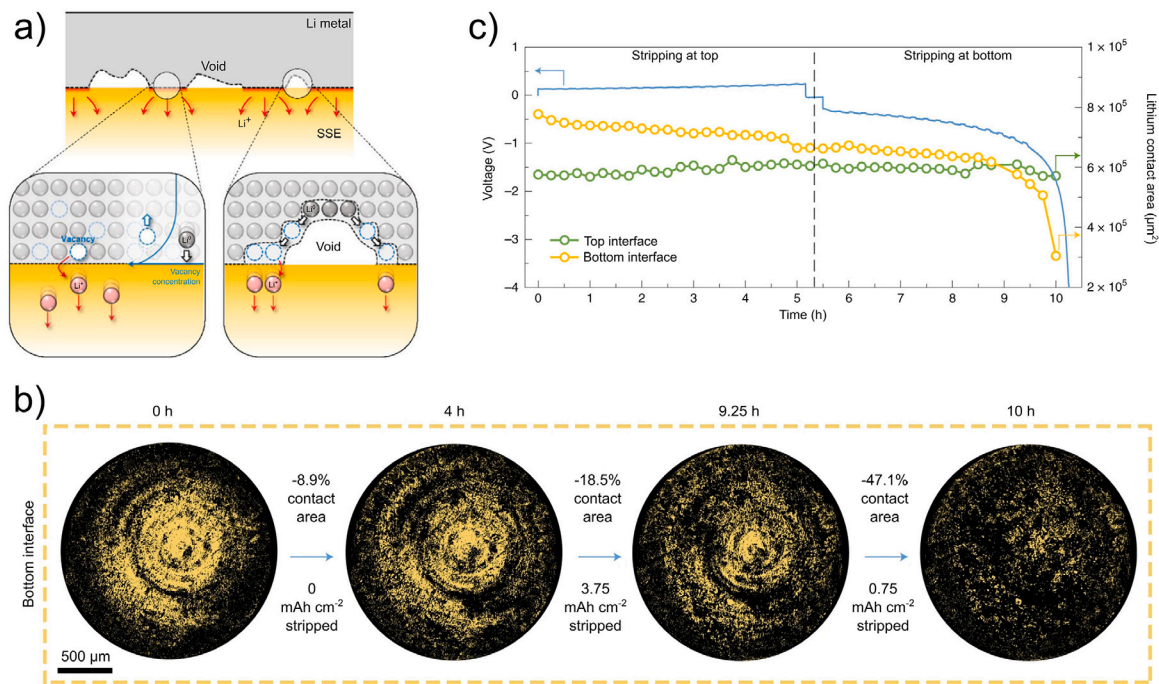
Fig. 16. (a) Schematic of the anode/SSE contact mechanics during dissolution, for a Li metal/SSE interface. (b) In operando X-ray computed tomography results in terms of Li/SSE interfacial contact. Colored pixels delineate contact regions, while black pixels indicate a lack of contact. (c) Contact area variations corresponding to (b), with yellow points. Image adapted from [477], © 2021, with permission from Springer Nature.
