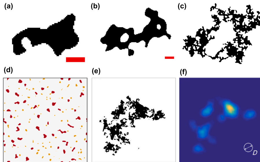
Fig. 2. Contact morphology and wear models. Contact islands in rough elastic contacts form fractal morphology with complicated branched structures. Panels (a) to (c) show contact islands of different size obtained from a multi-billion degrees-of-freedom boundary-element calculation. Adapted from Ref. [34], licensed under CC-BY 4.0. Such calculations have recently been used to formulate wear models. Panel (d) shows the selection of wearing contact based on a critical junction-size model, where red-islands have junction sizes that would wear. Adapted from Ref. [30], licensed under CC-BY 4.0. Panel (e) shows a contact morphology in combination with a color-code map (f) of energy released when a hypothetical half-sphere of diameter D is removed from the contact, also obtained from boundary-element calculations. Reprinted from Ref. [40], licensed under CC-BY 4.0.
