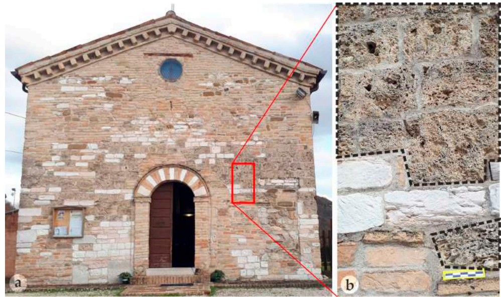
Figure 8. (a) Santa Barbara church (from the end of 12th to 14th century) partially built using calcareous tufas highlighted in the inset (b).
