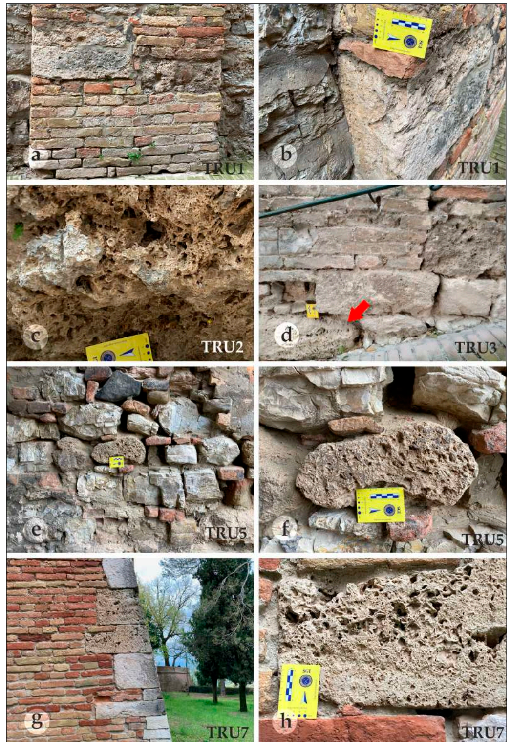
Figure 3. Blocks of calcareous tufas of the Roman period reused in some historical palaces (a–f) and Fortezza Alborno (g,h). Places are located in Figure 1 and reported in Table 1 according to the label numbers (TRU).
