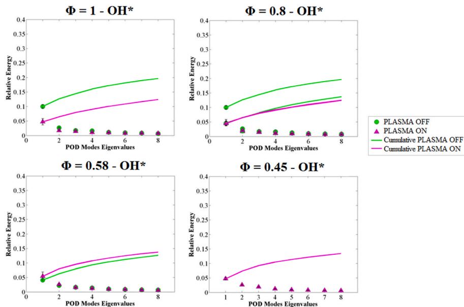
Fig. 5. Relative and cumulative energy contributions of the first eight POD modes extracted from OH* chemiluminescence images for \Phi = 1, 0.8, 0.58 , and 0.45 , with plasma OFF and ON. Error bars indicate the 95% confidence intervals estimated through bootstrap resampling of the temporal POD coefficients.
