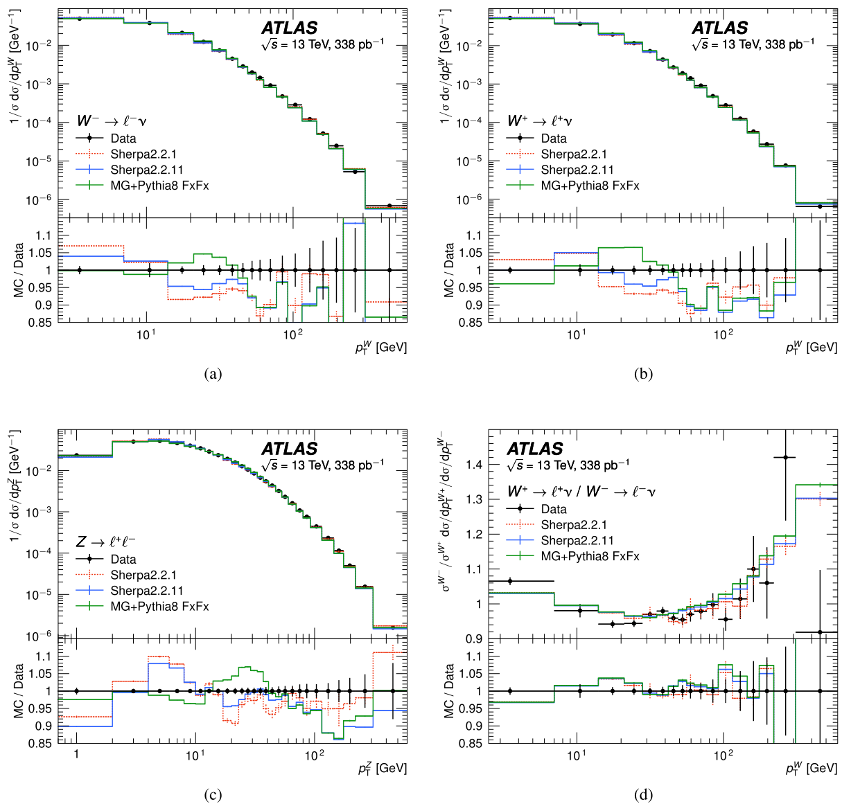
Fig. 31 Measurements of normalised differential distributions at \sqrt{s} = 13 TeV (black points) for a W^- , b W^+ , c Z as well as d the W^+ / W^- ratio compared to a variety MC predictions of multijet-merged NLO SHERPA and MADGRAPH_AMC@NLO FxFx+PYTHIA 8 samples
