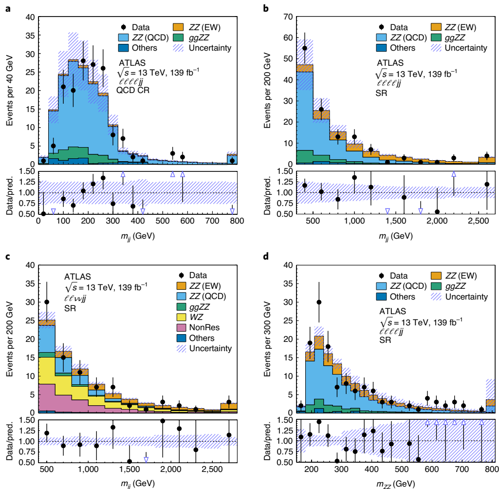
Fig. 2 | Observed and expected distributions. a–d , The m_{jj} distributions in the lllljj QCD CR ( a ) and the lllljj ( b ) and llvjj SRs ( c ), as well as the m_{zz} distribution in the lllljj SR ( d ). The error bands represent the s.d. and include the expected experimental and theoretical systematic uncertainties. The contributions from the QCD and EW production of ZZjj events are scaled by 0.99 and 0.92, respectively, which correspond to the observed normalization factors in the statistical fit to the combined channel (Table 2). ZZ (EW), ZZ (QCD) and ggZZ
