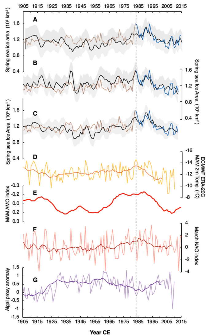
Fig. 4. Twentieth century sea ice reconstruction in the Baffin Bay and Labrador Sea. Black curves represent our reconstruction of the spring sea ice area based on \text{Br}_{\text{enr}} records from (A) SIGMA-A, (B) NU, and their compiled record (C). The statistical uncertainty is represented in gray with traditional 95 % prediction intervals. Solid blue lines represent the MAM sea ice area derived from satellite observations (1984-onward) while the dashed orange line is the reconstruction provided by Walsh et al. (2019). (D) Yellow curve represents 2 m air temperature from ECMWF-ERA20 reanalysis with 10-y moving average (orange). Values are averaged across 50–82 N and 80–45 W. (E) Red curve is the Atlantic Multi-decadal Oscillation (AMO) index (10-yr lowpass) based on Trenberth and Shea (2006), from CAS, NCAR. (F) March NAO index with a 10-y moving average (dark red) and (G) algal proxy record from Halfar et al. (2013) with 10-y moving average (violet). Lower values indicate more extended sea ice conditions.
