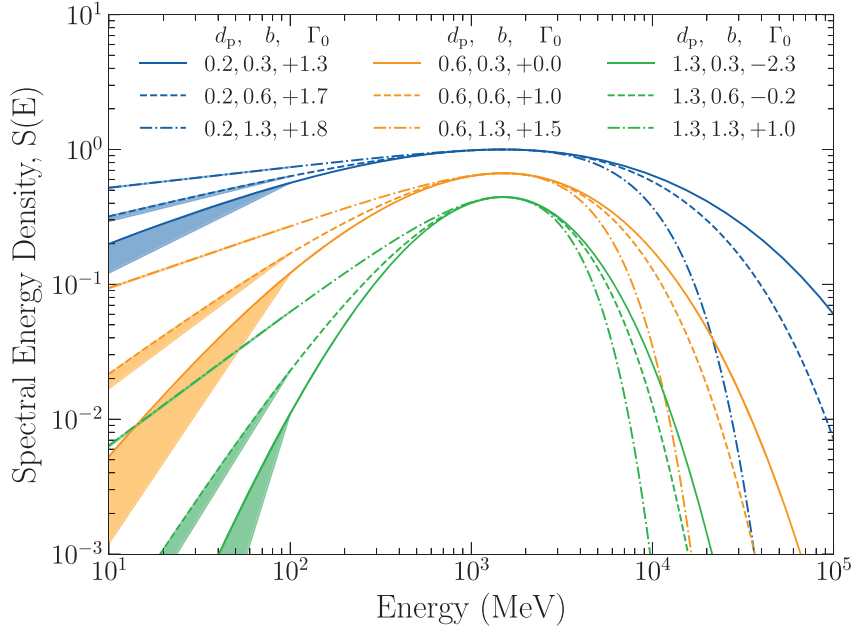
Figure 15. Realizations of the PLEC4 model for three values of the peak curvature, d_p = 0.2, 0.6, and 1.3, and the asymmetry parameter b = 0.3, 0.6, and 1.3. We set E_p = E_0 = 1 GeV, which uniquely determines \Gamma and \Gamma_0. The SEDs are normalized to 1 at E_p but offset by 50% for clarity. Each curve is labeled with the tuple (d, b, \Gamma_0). The shaded regions show the difference between the SED and the asymptotic power law, normalized to 0.1 GeV.
