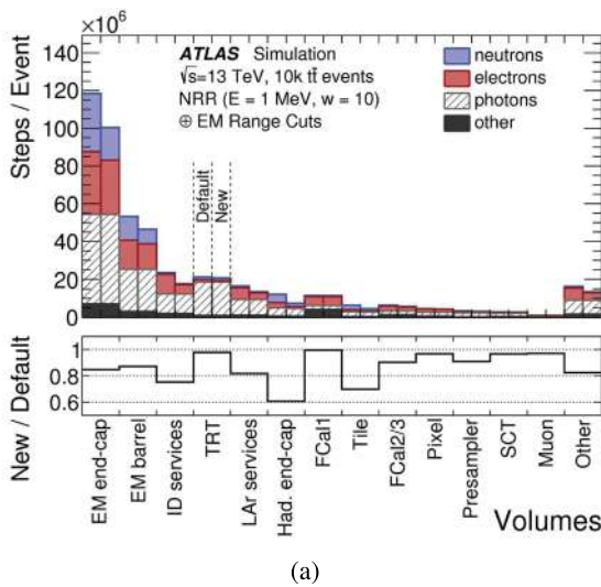
Fig. 7 a Average number of GEANT4 steps per event as a function of the subsystem in the Run 2 setup (MC16 production). b CPU time per event for various thresholds of the NRR algorithm relative to the
