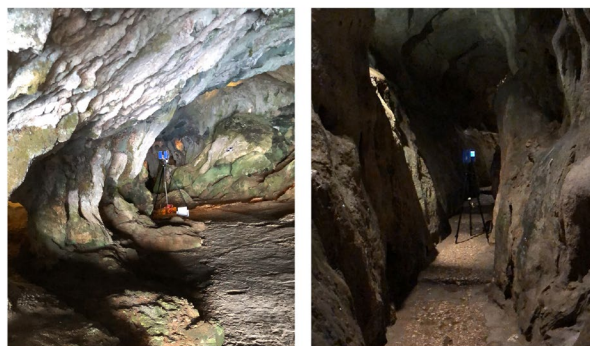
Figure 6. Tight and narrow indoor spaces of Grotta Zinzulusa.
