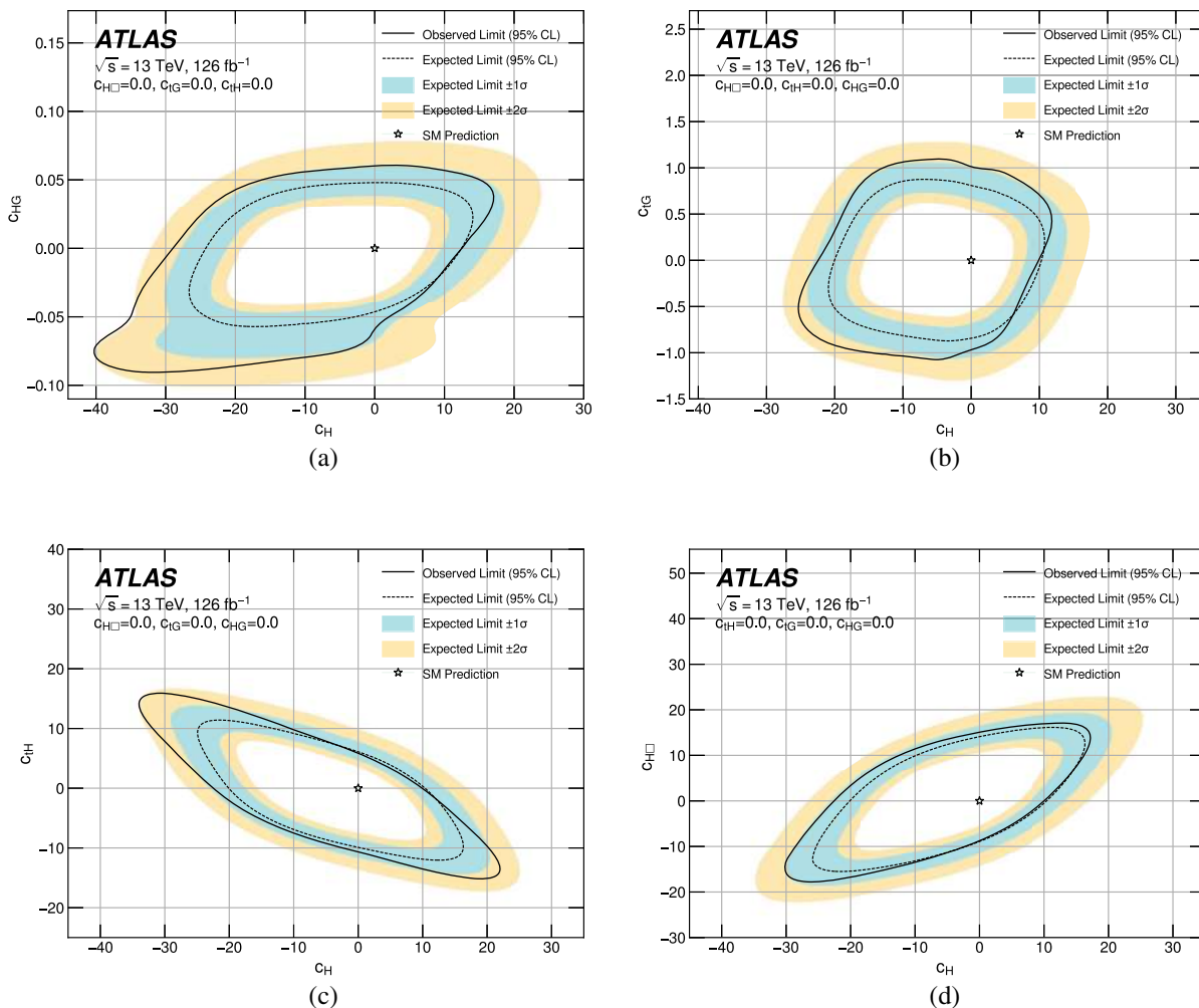
FIG. 14. The observed 95% CL exclusion limits on the SMEFT coefficients in the two-dimensional spaces (a) c_{HG} vs c_H , (b) c_{tG} vs c_H , (c) c_{tH} vs c_H , and (d) c_{H\Box} vs c_H , shown by the solid black lines. The dashed black line indicates the expected 95% CL exclusion limits. The shaded blue band indicates the \pm 1\sigma uncertainty of the exclusion limits, while the yellow band indicates the \pm 2\sigma uncertainty. The values of the other three coefficients for each plot are fixed to 0. The VBF HH process is ignored for this result.
