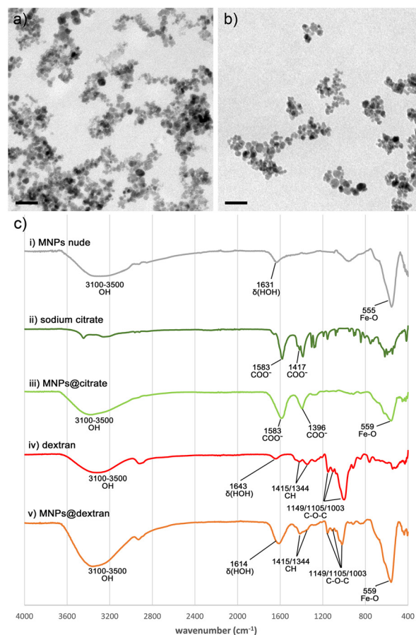
Fig. 3 TEM images of dextran-coated MNPs 20. Panel (a) shows a non-filtered MNP preparation, whereas panel (b) shows 0.1 \mu\text{m} filtered MNPs 20. The filtration step was added to remove any possible aggregate from the suspension. All scale bars correspond to 50 nm: (c) ATR-FTIR spectra of (i) nude MNPs, (ii) sodium citrate, (iii) citrate-coated MNPs, (iv) dextran and (v) dextran-coated MNPs.
