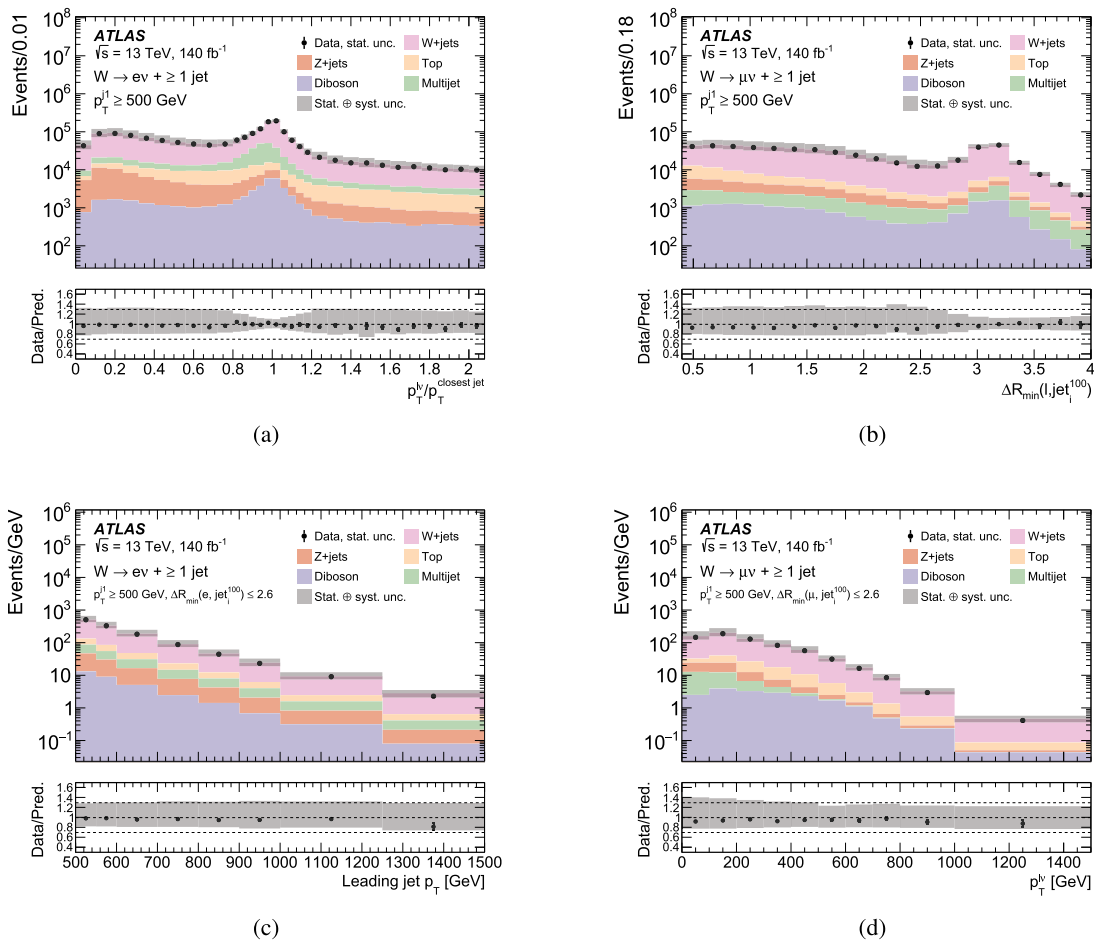
Fig. 2 Differential distributions at reconstruction level in the a, c electron and b, d muon channel for a, b inclusive and c, d collinear signal regions after the application of the background normalisation factors. The signal process is stacked above all background predictions. The
