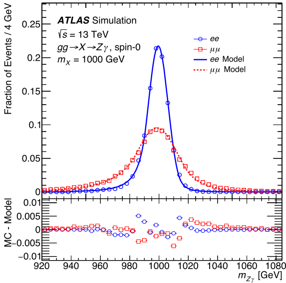
Fig. 2. Differential distributions of the invariant mass m_{Z\gamma} of the spin-0 resonance with m_X = 1000 GeV produced by the gluon-gluon fusion process. The markers show the distributions of the simulated events. The solid and dashed lines are the fitted models in the ee\gamma and \mu\mu\gamma channels, respectively. The mass resolution in the muon channel is compatible to that in the electron channel when m_X < 300 GeV.
