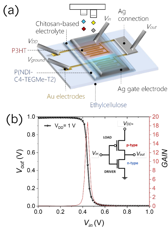
Fig. 5. (a) Schematic representation of the inverting logic gate device, realized with chitosan gated transistors based on P3HT and P(NDI-C4-TEGMe-T2); L = 10 \mu\text{m} , W = 10\,000 \mu\text{m} for p-type device and L = 30 \mu\text{m} , W = 10\,000 \mu\text{m} for n-type device. (b) Complementary inverter voltage transfer curve (VTC), and corresponding derivative curve to extract gain, as a function of input voltages; the sweep rate is 15 \text{ mV/s} ; the inverter configuration is reported as an inset.
