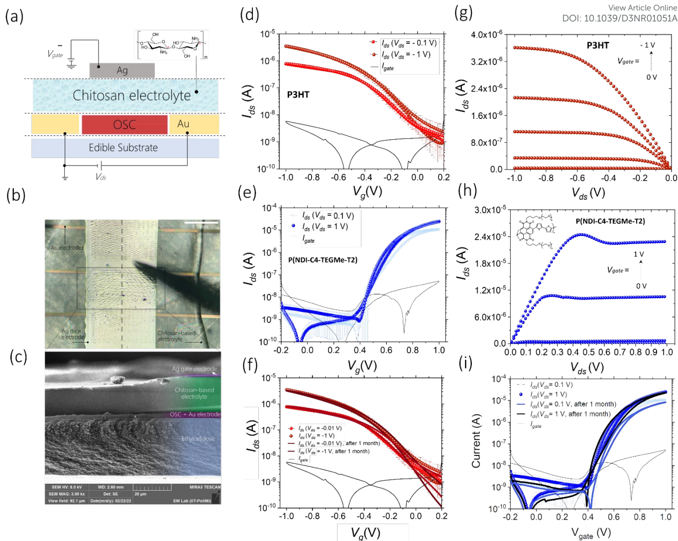
Fig. 4. Structure, fabrication, and electrical characterization of fully printed chitosan-gated transistors on edible substrate. (a) Schematic structure representation of the device. Chitosan chemical structure is shown in the inset. (b) Microscope image of three fully printed chitosan-gated transistors on ethylcellulose substrate with a common silver gate electrode (top view). The dashed line indicates the cross-section imaged via SEM (c) . It is possible to distinguish the layers composing the device: ethylcellulose substrate (30 \mu\text{m} ), a layer of semiconductor deposited on gold source and drain electrodes, chitosan-based electrolyte (15 \mu\text{m} ), and silver gate electrode. The layer of the semiconducting polymer was printed approximately 10 times thicker than in the actual device to help distinguish it in the stack of other layers. (d) Transfer and (e) output characteristic curves of the p-type fully printed chitosan gated transistors on ethylcellulose substrate in linear ( V_{ds} = -0.1 V) and saturation ( V_{ds} = -1 V) regimes (average curve over 7 samples); V_{gate} sweep rate was 5 mV/s. (f) Transfer and (g) output characteristic curves of the n-type fully printed chitosan-gated transistors on ethylcellulose substrate in linear ( V_{ds} = 0.1 V) and saturation ( V_{ds} = 1 V) regimes (average curve over 7 samples); V_{gate} sweep rate was 2 mV/s. Shelf-life stability of (h) the p-type and (i) the n-type fully printed chitosan gated transistors. The comparison between electronic performances (transfer characteristics in linear and saturation regimes) after a 1-month control period of storing the devices in air are shown.
