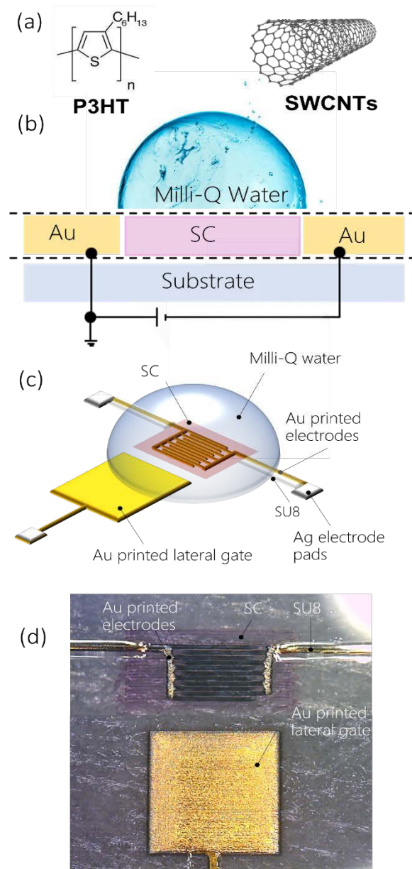
Fig. 2 (a) Chemical structure of the semiconducting materials adopted (P3HT and SWCNTs). (b) Schematic cross-section and (c) representation of the fully printed WGFET. (d) Microscope image of the device on a PEN substrate.
