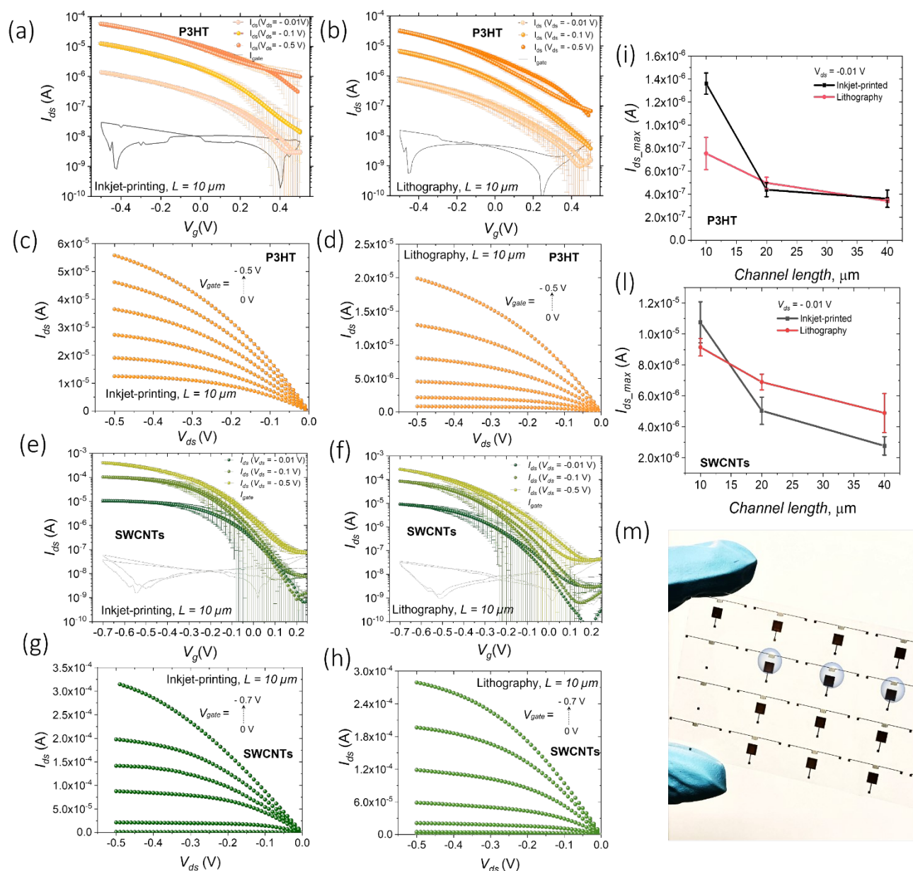
Fig. 3. Electrical characterization of WGFETs. (a) Transfer and (c) output characteristic curves for P3HT-based WGFETs with inkjet-printed gold electrodes, and (b) transfer and (d) output curves of devices with photolithographically patterned gold electrodes in linear ( V_{ds} = -0.01 V; -0.1 V) and saturation ( V_{ds} = -0.5 V) regimes; V_{gate} sweep rate was 10 mV/s; transfer curves are averaged over 7 samples; WGFETs geometrical parameters: L = 10 \mu\text{m} ; W = 10^5 \mu\text{m} . (e) Comparison of max I_{ds} for two different configurations of P3HT-based WGFETs (based on inkjet-printed and photolithographically patterned gold electrodes) in linear regime ( V_{ds} = -0.01 V) for devices with different channel lengths: L = 10 \mu\text{m} , L = 20 \mu\text{m} , L = 40 \mu\text{m} . (f) Transfer and (g) output characteristic curves for s-SWCNT-based WGFETs, with inkjet-printed gold electrodes, and (h) transfer and (i) output curves for devices with photolithographically patterned gold electrodes in linear ( V_{ds} = -0.01 V; -0.1 V) and saturation ( V_{ds} = -0.5 V) regimes; V_{gate} sweep rate was 10 mV/s; transfer curves are averaged over 7 samples; OFETs geometrical parameters: L = 10 \mu\text{m} ; W = 10^5 \mu\text{m} . (j) Comparison of max I_{ds} for two different configurations of s-SWCNT-based WGFETs (based on inkjet-printed and photolithographically patterned gold electrodes) in linear regime ( V_{ds} = -0.01 V) for the devices with different channel lengths: L = 10 \mu\text{m} , L = 20 \mu\text{m} , L = 40 \mu\text{m} . (m) Digital image of the WGFETs.
