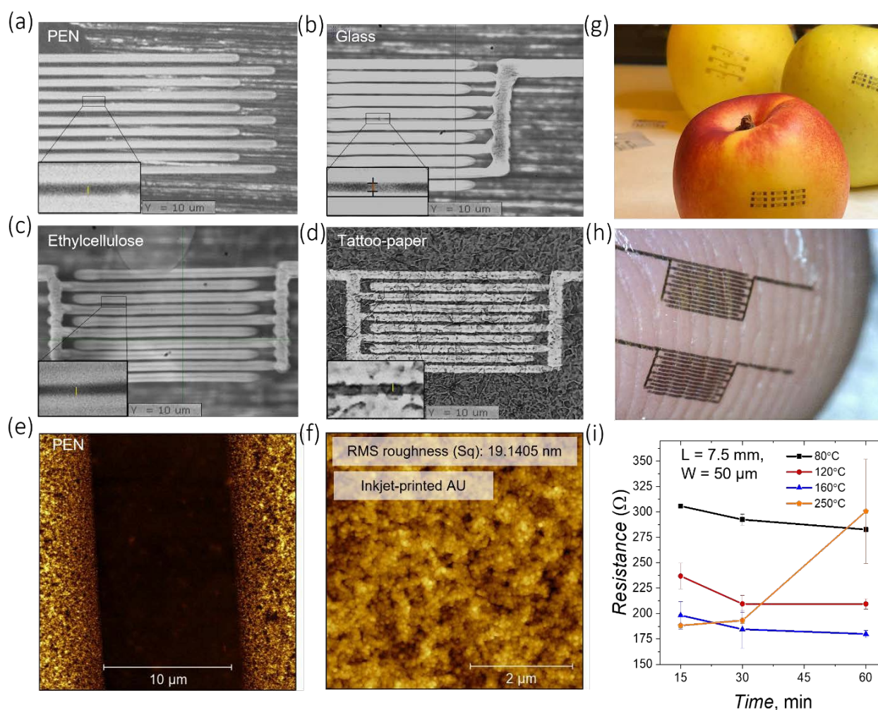
Fig. 1. Structural, morphological, and electrical characterization of inkjet-printed gold electrodes on different conventional and edible substrates. (a) – (d) Gold interdigitated electrodes inkjet-printed on different substrates: PEN, glass, edible ethyl cellulose and tattoo-paper substrates. (g), (h) Digital photograph of gold electrodes transferred onto different surfaces: (top) a peach, an apple and (bottom) a fingertip. (e) AFM of gold electrodes inkjet-printed on PEN: topography of the area between the two conducting fingers of the interdigitated electrodes with a channel length of 10 μm; the area of the image is 20x20 μm 2 . (f) AFM topographic image of the top surface of the gold electrode. The image area is 5x5 μm 2 . (i) Dependence of electrical resistance of inkjet-printed gold lines on drying conditions. The plots are presented for lines with a length of 7.5 mm. Each point corresponds to the average value measured over 7 samples.
