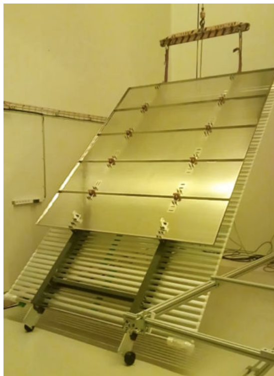
Figure 18. Lifting of a Top FC module for subsequent installation on the CPA panel. The side of the FC module that is lifted will attach to the CPA while the other side (bottom side) is connected with latches to the APA.
