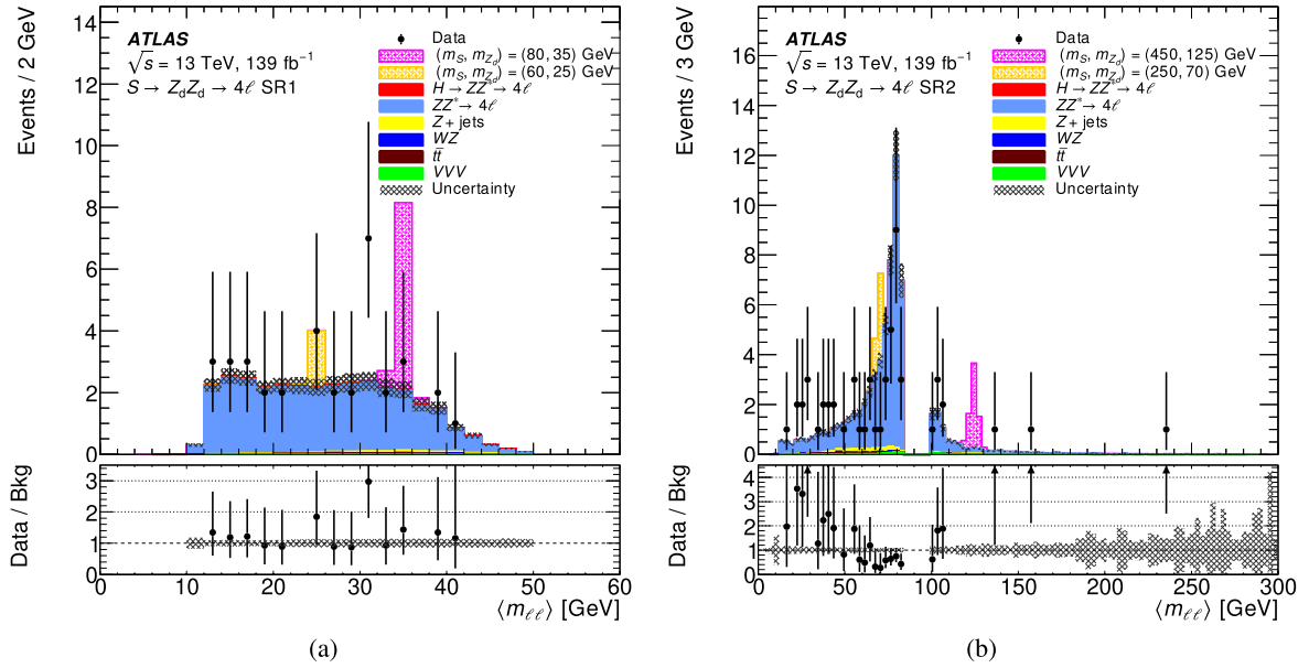
Fig. 1. Distributions of the average dilepton mass \langle m_{\ell\ell} \rangle = \frac{1}{2} (m_{ab} + m_{cd}) for the two signal regions (a) SR1 and (b) SR2. The hatched bands show the uncertainty in the background prediction. The uncertainties on the data points are asymmetric Poisson errors (Eqs. (40.82a) and (40.82b) of Ref. [62]). The lower panels show the ratio of the observed data to the background ('Bkg') predictions. The arrows at the upper edge indicate data points that fall outside of the y-axis range, and the plotted uncertainties include both the Poisson errors on the data and the uncertainty on the background prediction. Distributions for two example signal points are also shown. These are normalized to production cross sections of 0.5 fb for SR1 and 0.1 fb for SR2.
