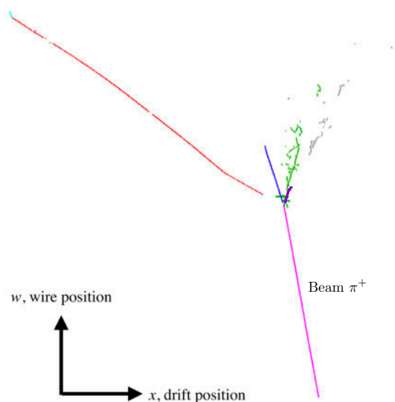
Figure 26. A reconstructed, simulated test-beam interaction showing the incoming beam \pi^+ track in magenta and a number of secondary particles created at the interaction vertex. The different colors represent different reconstructed particles.
