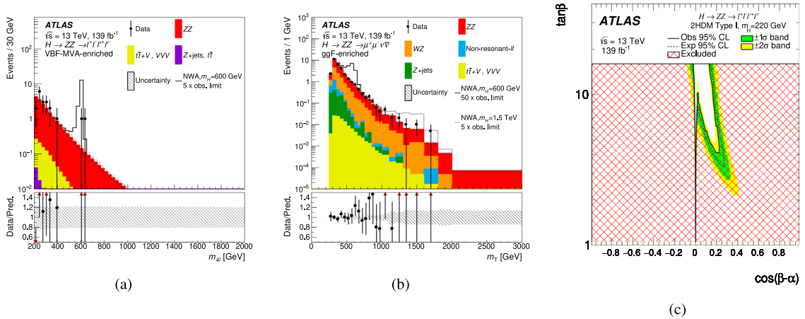
Fig. 20. H \rightarrow ZZ : (a) The mass reconstructed from the four leptons in the VBF-enriched category. (b) The transverse mass in the ggF category. In both mass plots, various signal hypotheses are overlaid for illustration. (c) The 95% CL exclusions in a type-I 2HDM for a heavy scalar mass of 220 GeV. Source: Figures are taken from Ref. [78].
