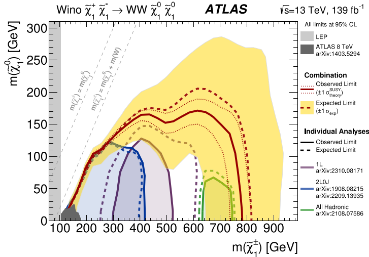
Fig. 13. The exclusion limits on \tilde{\chi}_1^+ \tilde{\chi}_1^- production with W -boson-mediated decays, as a function of the \tilde{\chi}_1^\pm and \tilde{\chi}_1^0 masses. The production cross-section is for pure-wino \tilde{\chi}_1^+ \tilde{\chi}_1^- . The labels with L and J denote the number of leptons and jets in the search, respectively. Where more than one reference is given for each line, the total exclusion limit from multiple analyses is shown.
