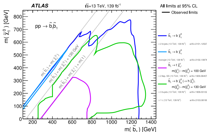
Fig. 9. Exclusion limits in the m(\tilde{b}_1)-m(\tilde{\chi}_1^0) plane for direct sbottom production. The lightest neutralino ( \tilde{\chi}_1^0 ) is assumed to be the LSP. Several different decay scenarios are shown, along with different parameterisations of the intermediate particles in the models. Where more than one reference is given for each line, the total exclusion limit from multiple analyses is shown.
