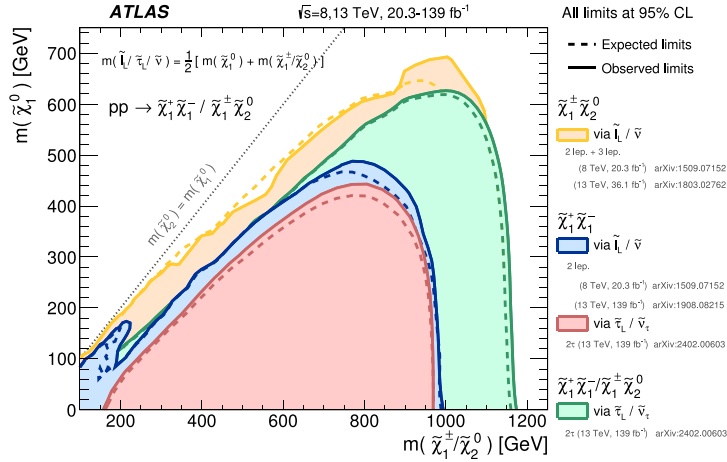
Fig. 12. The exclusion limits on \tilde{\chi}_1^+ \tilde{\chi}_1^- and \tilde{\chi}_1^\pm \tilde{\chi}_2^0 production with \tilde{l} -mediated decays, as a function of the \tilde{\chi}_1^\pm , \tilde{\chi}_2^0 and \tilde{\chi}_1^0 masses. The production cross-section is for pure-wino \tilde{\chi}_1^+ \tilde{\chi}_1^- and \tilde{\chi}_1^\pm \tilde{\chi}_2^0 . Where more than one reference is given for each line, the total exclusion limit from multiple analyses is shown.
