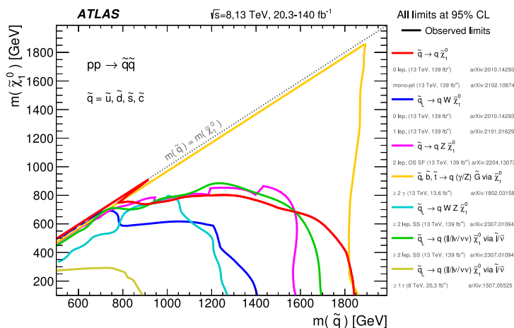
Fig. 8. Exclusion limits from 8 TeV and 13 TeV data in the m(\tilde{q})-m(\tilde{\chi}_1^0) plane for different simplified models featuring the decay of squarks to the lightest supersymmetric particle (lightest neutralino or gravitino) either directly or through a cascade chain featuring other SUSY particles with intermediate masses. For each line, the squark decay mode is reported in the legend and it is assumed to proceed with 100% branching fraction. The limits on \tilde{q}_L \rightarrow qW\tilde{\chi}_1^0 assume the chargino mass to be midway between the squark and neutralino masses. The other \tilde{q}_L interpretations assume the first intermediate particle to be midway between the squark and neutralino masses, and the second intermediate particle to be midway between the first intermediate particle and neutralino masses. The additional assumptions about the masses of the intermediate states are described in the references cited in the plot. Where more than one reference is given for each line, the total exclusion limit from multiple analyses is shown.
