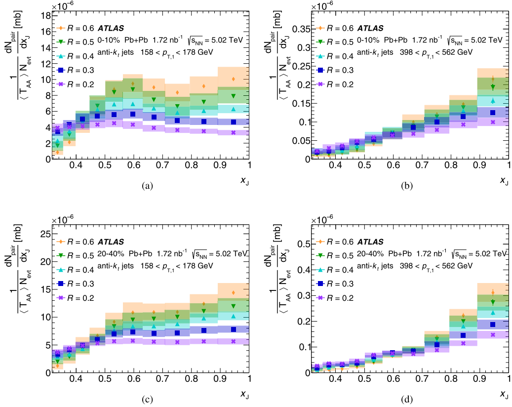
FIG. 12. The absolutely normalized x_1 distributions in (a), (b) 0–10% and (c), (d) 20–40% central Pb+Pb collisions, for leading jets with (a), (c) 158 < p_{T,1} < 178 GeV and (b), (d) 398 < p_{T,1} < 562 GeV. Jets are selected with |y| < 2.1 and |\phi_1 - \phi_2| > 7\pi/8 . The normalization uncertainties (not shown) are \delta\langle T_{AA} \rangle / \langle T_{AA} \rangle = 0.9\% and 2\% for Pb+Pb centrality selections 0–10% and 20–40%, respectively. The boxes correspond to systematic uncertainties and the bars to statistical uncertainties.
