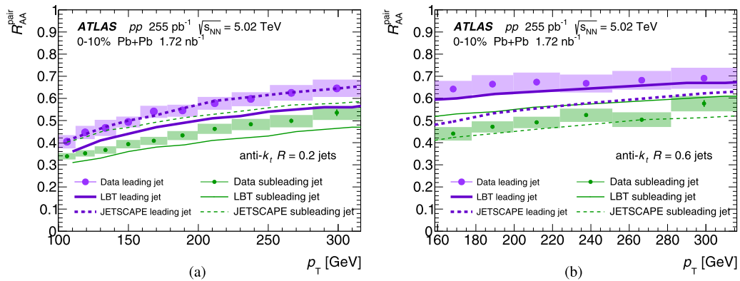
FIG. 19. The leading and subleading jet R_{AA}^{\text{pair}} distributions in dijets in data, compared with the LBT and JETSCAPE (LBT + MATTER) models. (a) R = 0.2 and (b) R = 0.6 jets are shown for 0–10% central collisions. Jets are selected with |y| < 2.1 and |\phi_1 - \phi_2| > 7\pi/8 . The normalization uncertainties in the data (not shown) are \delta\langle T_{AA} \rangle / \langle T_{AA} \rangle = 0.9\% in 0–10% Pb+Pb collisions and \delta L_{pp} / L_{pp} = 1\% in pp collisions. The boxes correspond to systematic uncertainties and the bars to statistical uncertainties.
