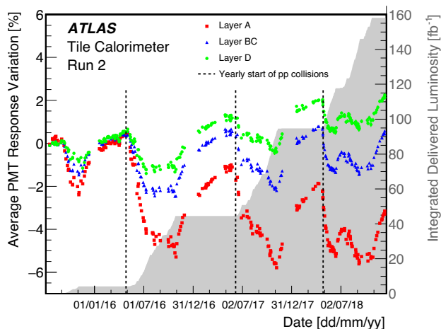
Fig. 12 The mean response variation \Delta R_{\text{Las}} in the PMTs for each layer, as a function of time, observed during the entire Run 2 (between standalone laser calibration runs taken on 17 July 2015 and 22 October 2018). For each layer, the response variation is defined as the mean of a Gaussian function fit to the response variations in the channels associated with given layer. Known bad channels are excluded. The LHC integrated delivered luminosity is shown by the shaded area
