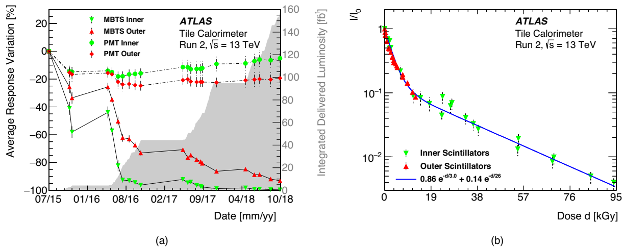
Fig. 21 a The average response variation of the MBTS inner (down triangles) and outer (up triangles) counters as a function of time during Run 2. The circle (diamond) markers show the relative response of the PMTs of the inner (outer) counters. The LHC delivered luminosity is shown by the shaded area. b The average relative light yield ( I/I_0 ) of scintillators and fibres of inner (down triangles) and outer (up triangles)
