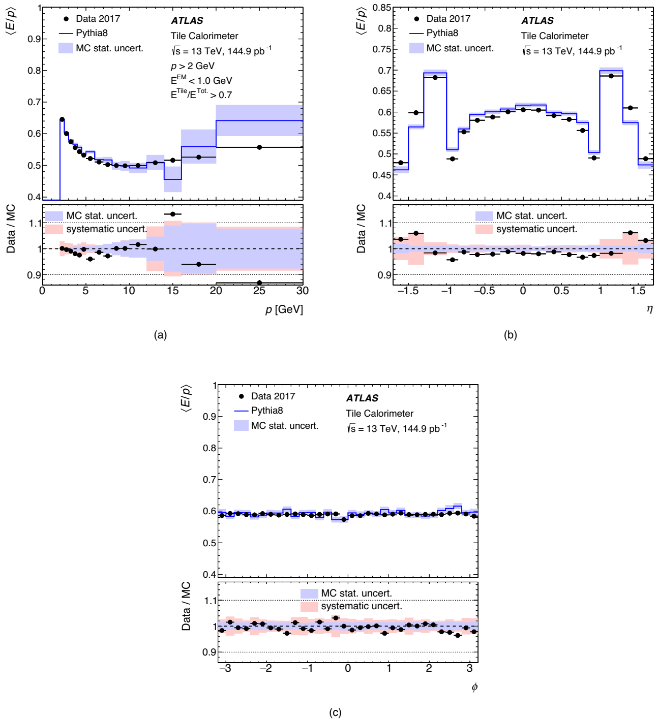
Fig. 27 The average ratio of energy to momentum ( \langle E/p \rangle ) measurements as a function of a momentum p , b pseudorapidity \eta and c azimuthal angle \phi . The ratios of experimental to simulated data are plotted in the lower panels. MC statistical and experimental systematic uncertainties are shown
