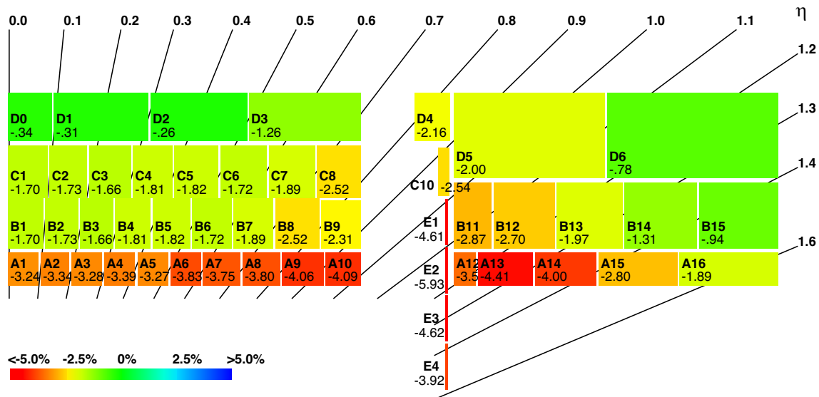
Fig. 11 The mean response variation \Delta R_{\text{Las}} in the PMTs for each cell type, in percent, averaged over \phi , observed during the entire pp collisions data-taking period in 2018 (between standalone laser calibration runs taken on 18 April 2018 and 22 October 2018). For each cell type,
