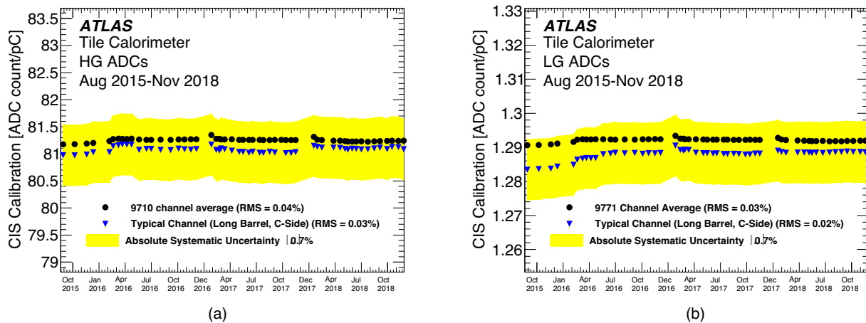
Fig. 7 The charge injection system constants ( C_{\text{ADC} \rightarrow \text{pC}} ) for the a high-gain and b low-gain ADCs, as a function of time, observed during the entire Run 2 (between CIS calibration runs taken on August 2015 and November 2018). Values for the average over all channels and for one typical channel are shown. The RMS values indicate the
