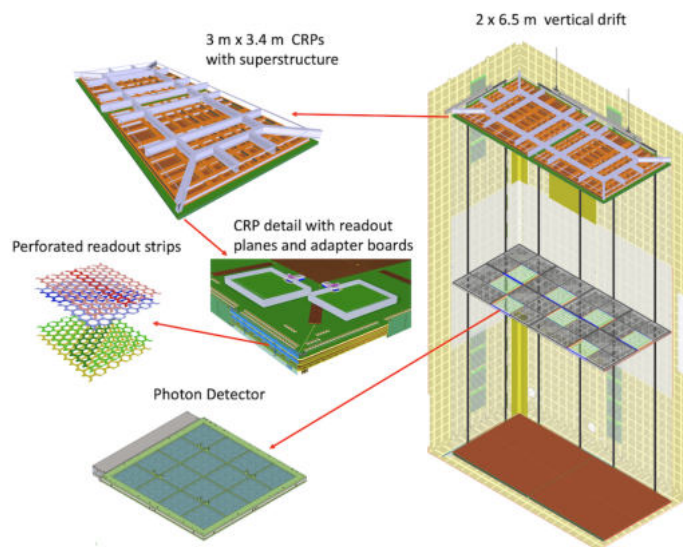
Figure 8. Schematic of the vertical drift FD2 concept with PCB -based charge readout. Corrugations on cryostat wall shown in yellow; PCB -based CRPs (brown, at top and bottom with superstructure in gray for top CRPs); cathode (violet, at mid-height with openings for photon detectors); field cage modules (white) hung vertically around the perimeter (the portions near the anode planes are 70% optically transparent); photon detectors (light green at right), placed in the openings on the cathode and on the cryostat walls, around the perimeter in the vertical regions near the anode planes. Reproduced from [60]. The Author(s). CC BY 4.0.
