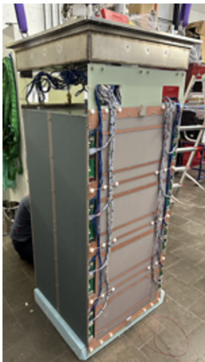
Figure 17. Left: a photograph of one of the four ton-scale LArTPC modules for the 2x2 Demonstrator, a prototype of the DUNE ND. Right: an example cosmic ray imaged in true 3D using a 102,400-channel LArPix-v2 system in this module (right).
