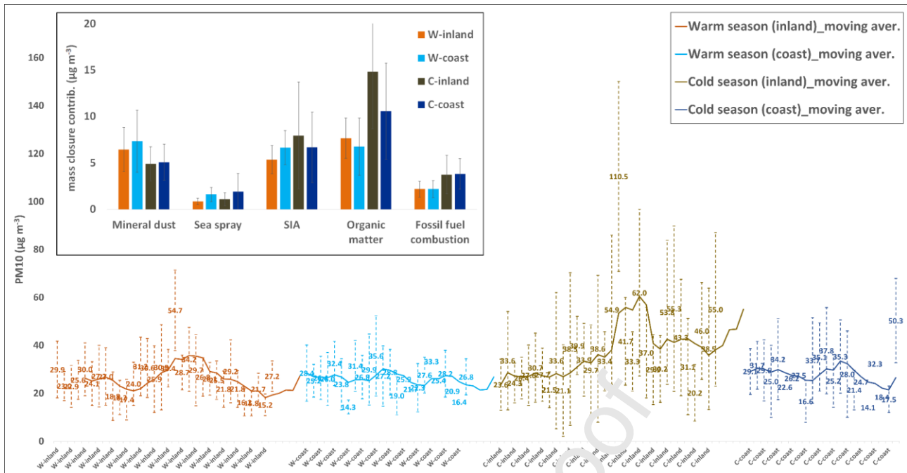
Figure 3. \text{PM}_{10} mean values reported by combining season (warm (W) / cold (C)) and proximity to coastline (inland/coast) site information. Error bars are standard deviation submitted with mean values. Lines are moving averages by a fixed subset of 5, for each group. The highest values in the W-inland, C-inland and C-coast groups refer to Milano in 2006 (54.7 and 111 \mu\text{g m}^{-3} ) and Napoli in 2015 ( 50.3 \mu\text{g m}^{-3} ), respectively. In the inner plot, \text{PM}_{10} contributions calculated by mass closure are also reported by combined criteria of season and proximity to coastline.
