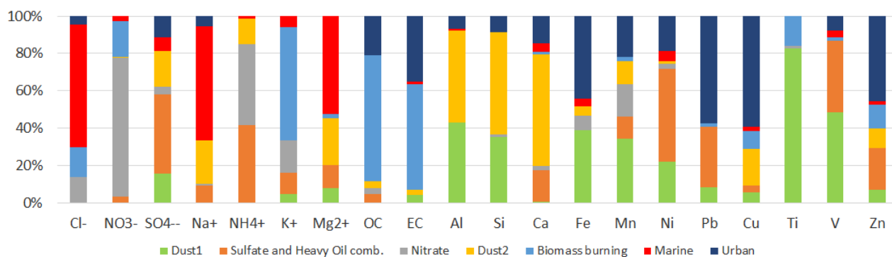
Figure 5. Sharing of chemical species (percent contributions) in the factor profiles extracted by the best PMF solution.
