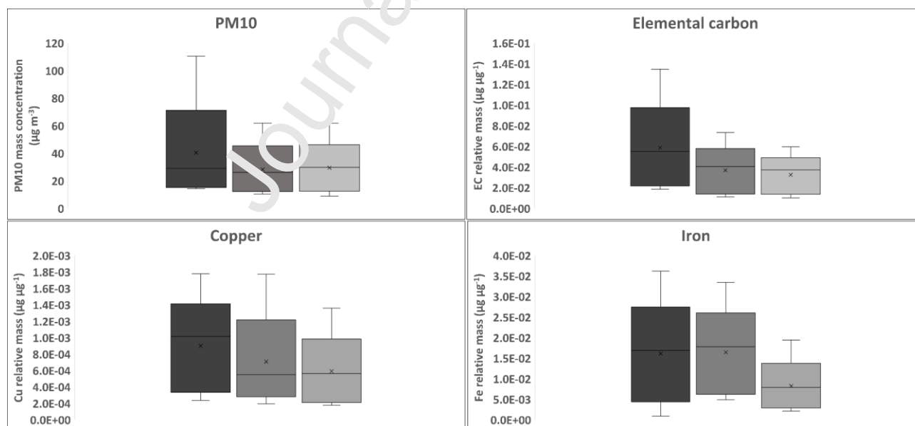
Figure 4. Box and whiskers plot of the species whose relative mass in the PM 10 is significantly discriminated among cities with different density of the general population (null hypothesis of similarity rejected by two-tailed Welch's t test, at 95% confidence level). For each species, cases are grouped by
