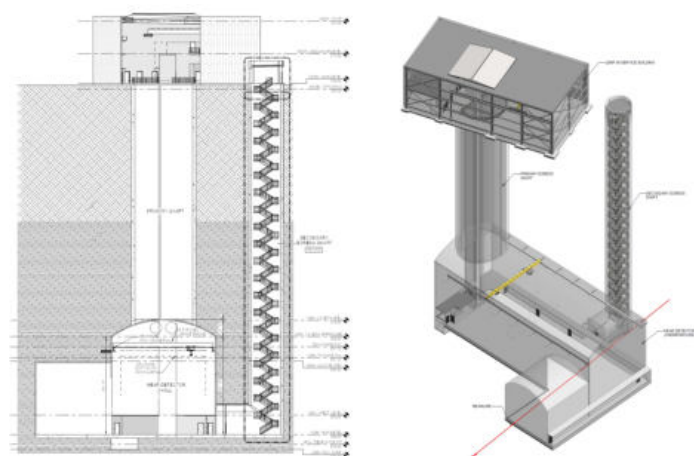
Figure 166. Near Detector cavern and surface building architectural drawings.
