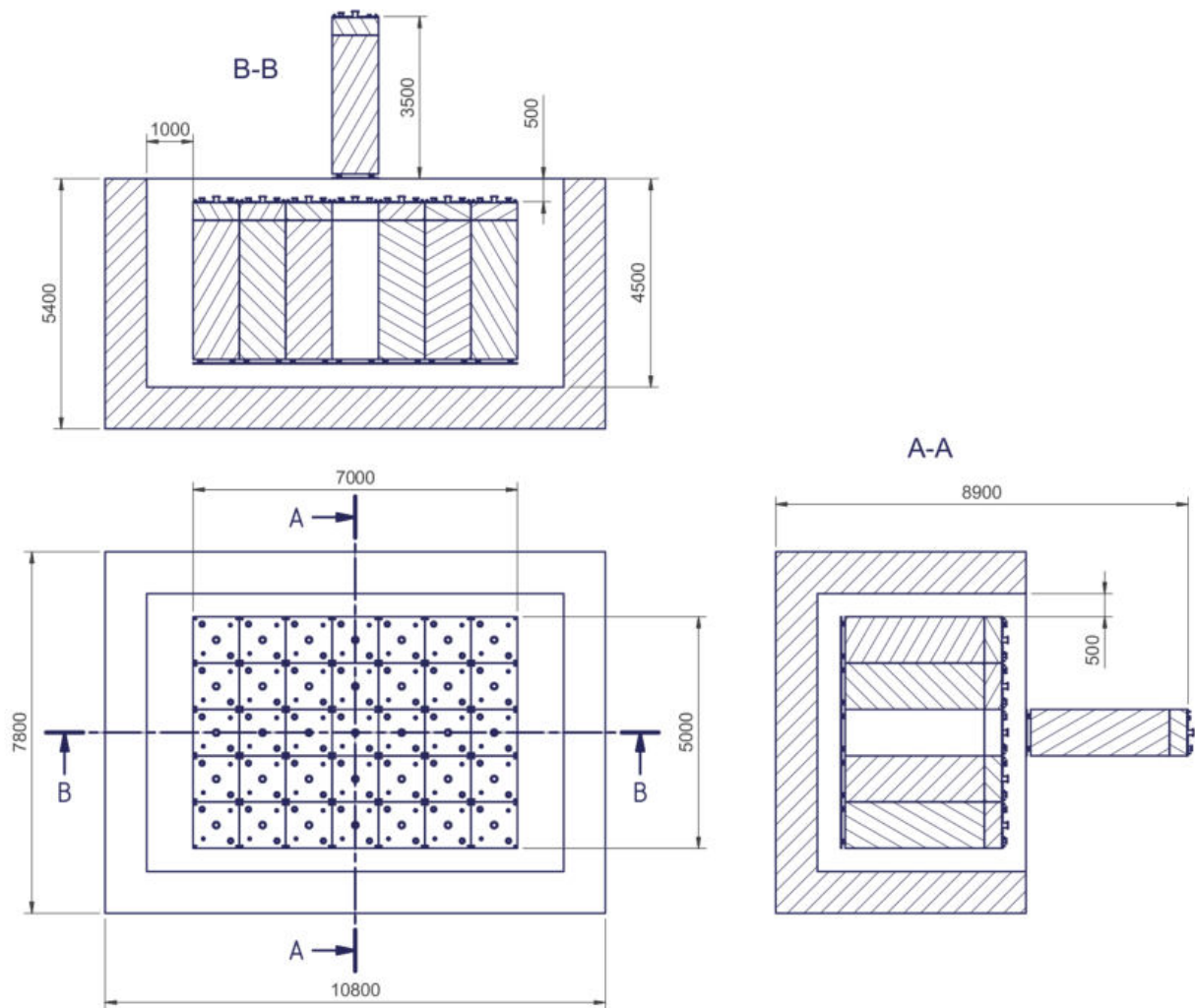
Figure 5. The current dimensions for the ArgonCube detectors in ND-LAr. The cryostat is based on the 35 ton prototype and ProtoDUNE [62], and is yet to be optimized for the DUNE ND. In this figure, the lower left is the top view, the upper plot is a view of a horizontal cut transverse to the beam, and on the lower right is a horizontal cut along the beam.
