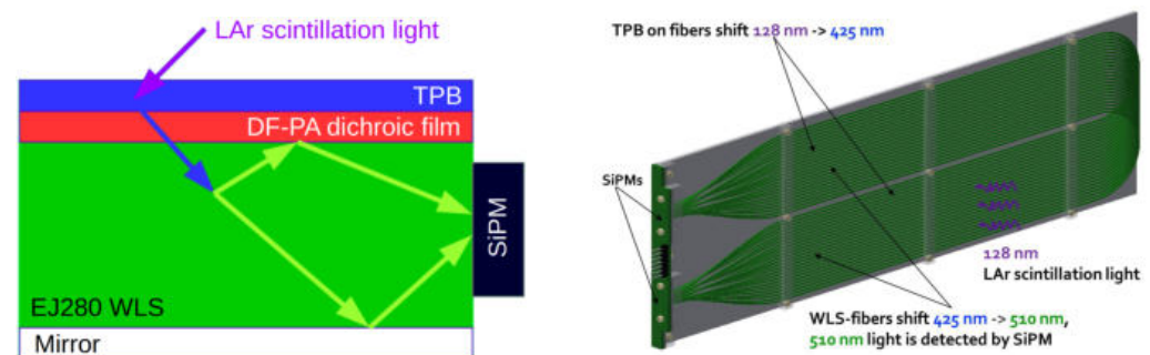
Figure 9. Two approaches to light detection: ArCLight (left) and LCM (right).
