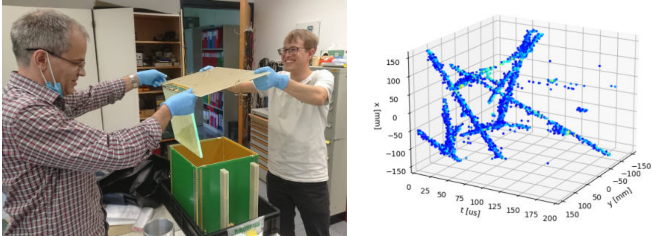
Figure 15. (Left) Installation of a LArPix tile and ArCLight panel assembly into the SingleCube TPC at the Univ. of Bern. (Right) An overlay of the raw data from 25 typical cosmic ray events collected during the first SingleCube operation run in October 2020.
