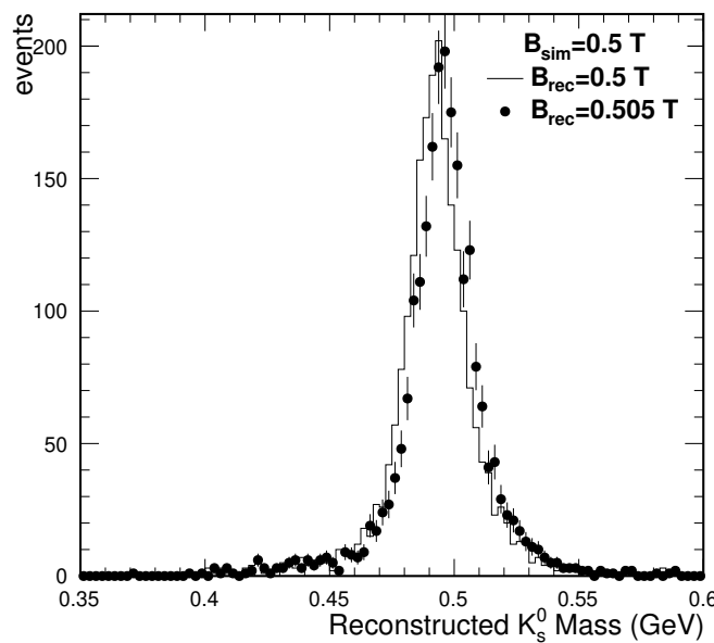
Figure 58. The invariant mass distribution for reconstructed K_s^0 \rightarrow \pi^+\pi^- decays. The K_s^0 were generated as single particle events inside the HPgTPC and then reconstructed in GARSoft with an efficiency of about 33%. The kaon mass ( m_{K0} = 497.6 MeV according to the PDG) is well reproduced by the mean of the distribution, and a 1% bias in the magnetic field (and therefore also in the momentum) results in a clear shift of the mean.
