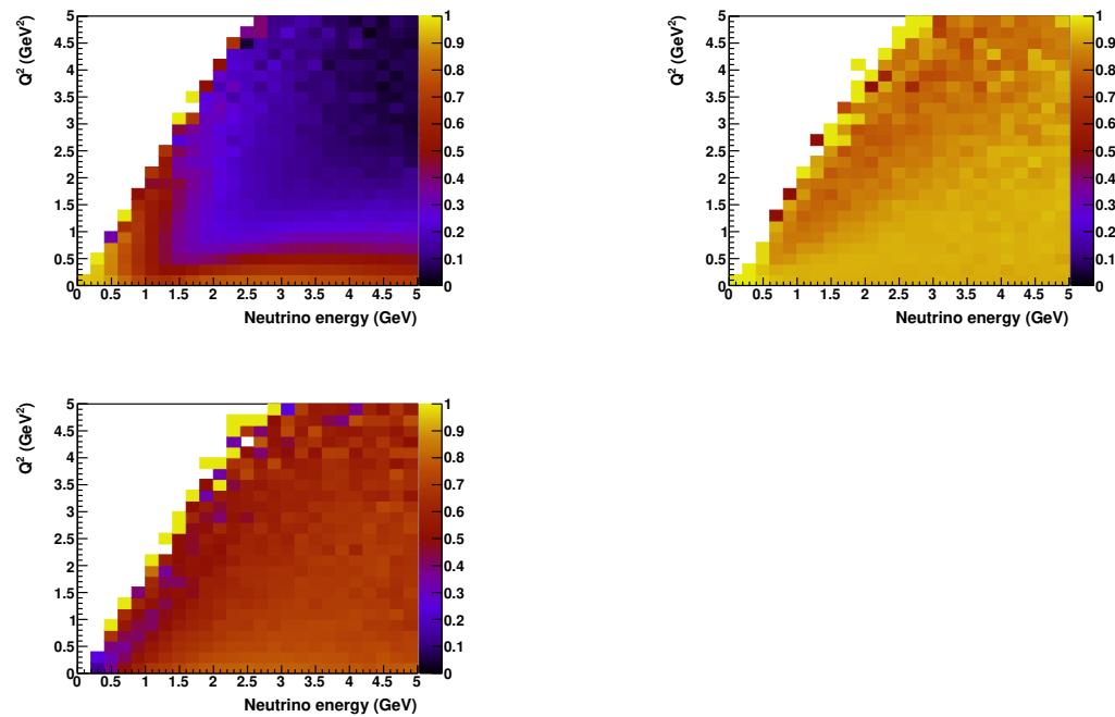
Figure 57. Comparison of the acceptance of ND-LAr (left), ND-GAr (middle), and the FD (right) for the range of neutrino energy and squared momentum transfer ( Q^2 ) of \nu_\mu CC interactions expected at DUNE. ND-GAr and the FD are well-matched in their acceptance of events across the range of phase space.
