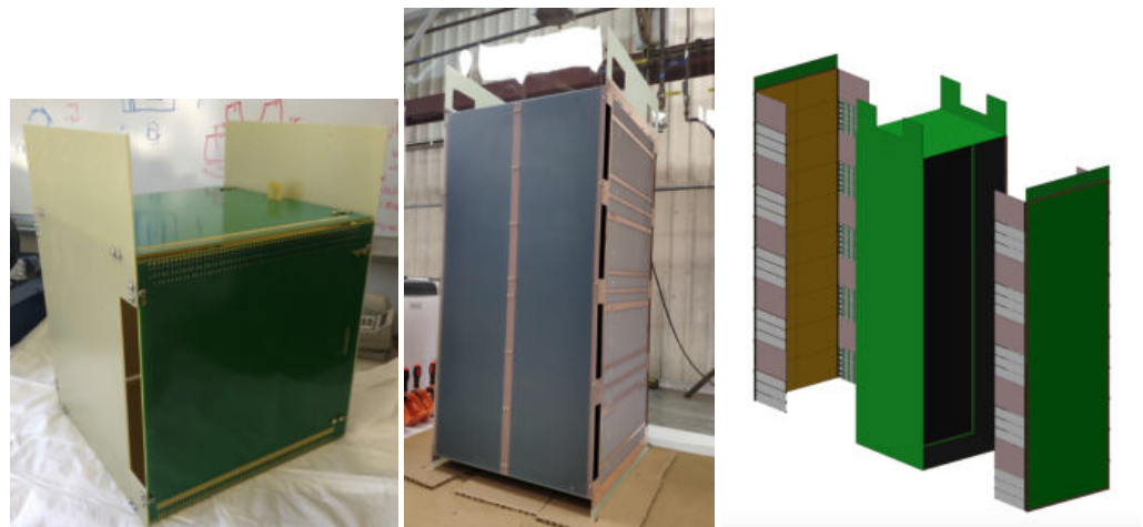
Figure 14. (Left) The SingleCube LArTPC designed to test a single integrated large-format charge and light readout element. (Center) The mechanical assembly of the first module (Module 0) of the ArgonCube 2 \times 2 Demonstrator, including the cathode, field cage, and anode support panels. The module is a sub-scale prototype of the ND LArTPC module, at 60% drift length and 40% module height. (Right) The engineering model of the full-scale ND LArTPC module (1 m by 1 m footprint and 3.5 m height), shown with the anode panels detached from the field cage. The pixelated anode tiles (gold rectangles) provide true 3D imaging, while the dielectric light traps (pink and white rectangles) provide high-efficiency scintillation light detection.
