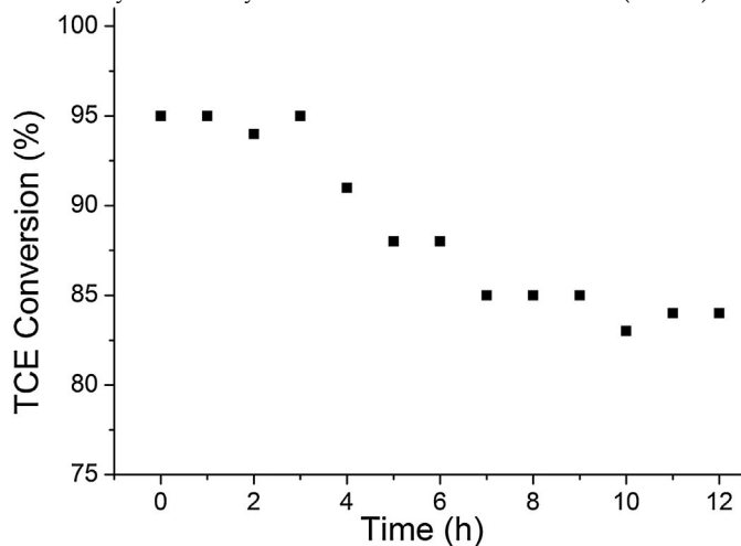
Fig. 5. Stability of the mayenite catalyst (reaction conditions: T_{95} = 500 °C, [\text{TCE}]_{\text{inlet}} = 1700 ppm, GHSV = 6000 \text{ h}^{-1} , 0.8 g of catalyst).
